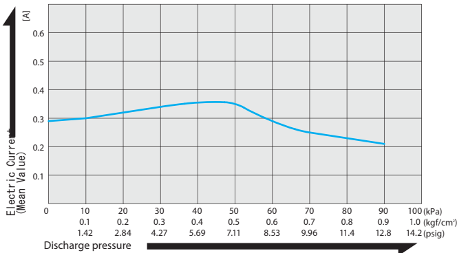
Current Characteristics
