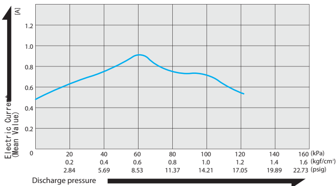
Current Characteristics
